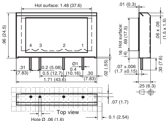
Figure 1 - LS relays; dimensions in inches (mm) (See Figure 12 for LS with HS1)
